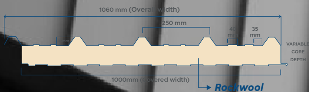
Mineral Wool / Rockwool Roof Panel (MRWRP)
